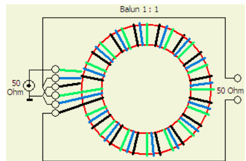
Winding scheme for a 1 \div 1 balun.
