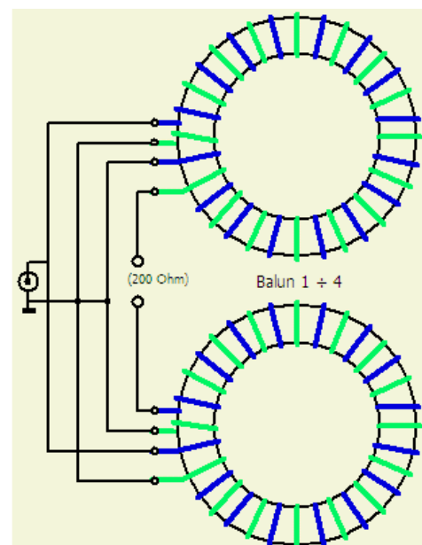
Winding scheme for a 1 \div 4 balun.
