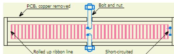
Stub made with Rolled up ribbon line.
