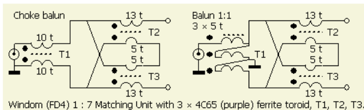
Windom (FD4) 1 : 7 Matching Unit with 3 × 4C65 (purple) ferrite toroid, T1, T2, T3.
