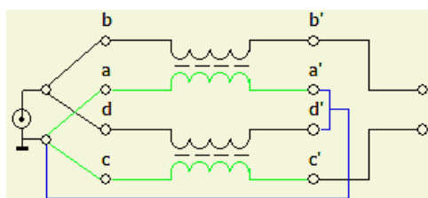
The principle of the 1 \div 4 system.
