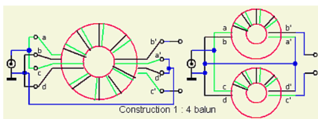
schemes for 1 \div 4 baluns.
