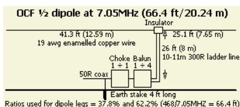
2EØZEH's version of an OCF.
