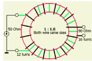
Winding scheme for a 1 ÷ 1.8 balun.
